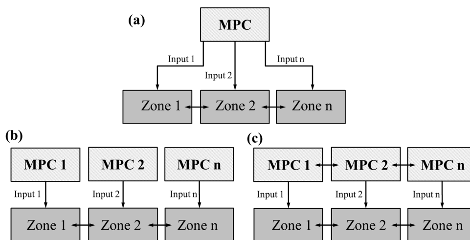
Figure 13. (a) Centralized MPC formulation; (b) decentralized MPC formulation; (c) distributed MPC formulation.
